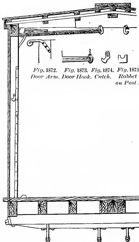
Fig. 1871. Half Cross Section.
